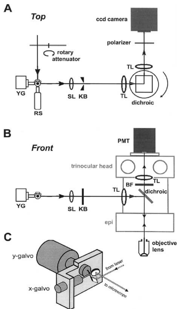
Fig. 2 (A, B) Schematic diagrams of the scan head and its coupling to the microscope viewed, respectively, from the top and front. SL = scan lens (10 \times widefield eyepiece); TL = tube lens; KB = variable knife-blade aperture; BF = barrier filter blocking laser light; epi = epi-illumination illuminator; dichroic = dichroic mirror reflecting \lambda > 650 nm, mounted in rotating housing. (C) Rendering of the scan head assembly.
